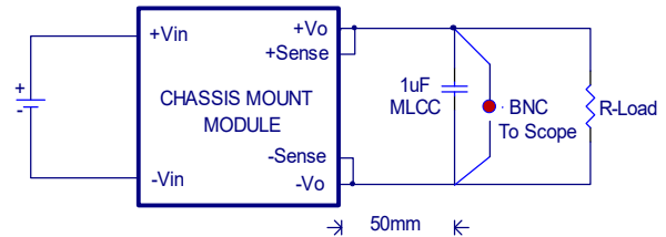
Output Ripple and Noise
