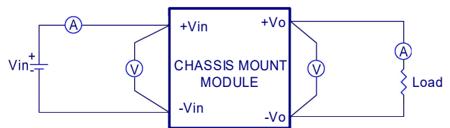
CFB750-300SXX-CMFD Series Test Setup
