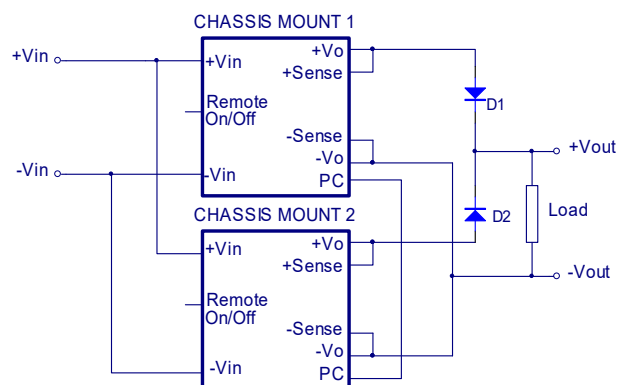
Simple Redundant Operation Connect Circuit
