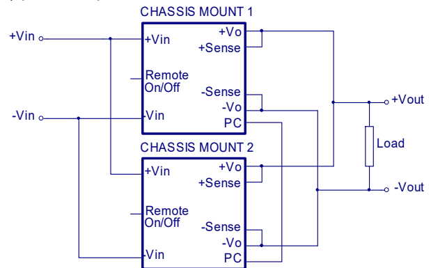
Simple Parallel Operation Connect Circuit
